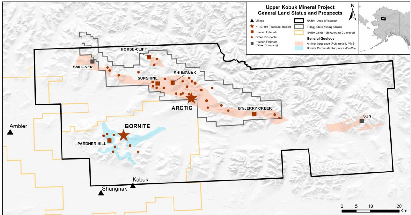
Figure 1: Upper Kobuk Mineral Projects, Alaska
