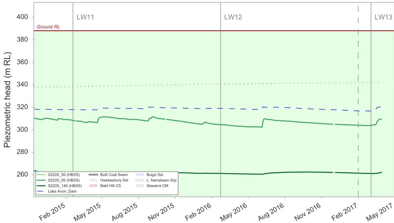
Figure 15. Hydrograph for vibrating wire piezometer S2220
