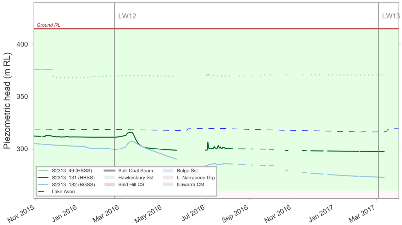
Figure 23. Hydrograph for vibrating wire piezometer S2313
