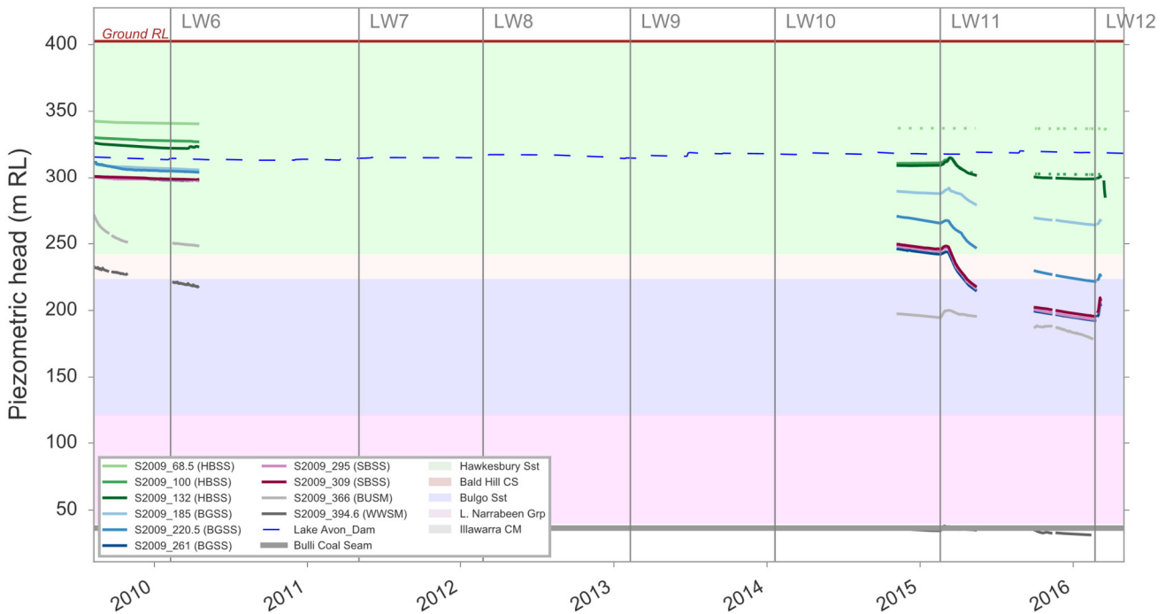
Figure 16. Hydrograph for vibrating wire piezometer S2009
