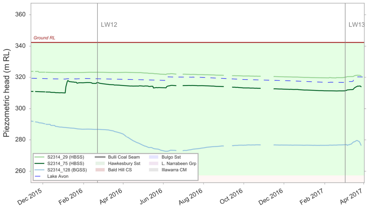
Figure 24. Hydrograph for vibrating wire piezometer S2314
