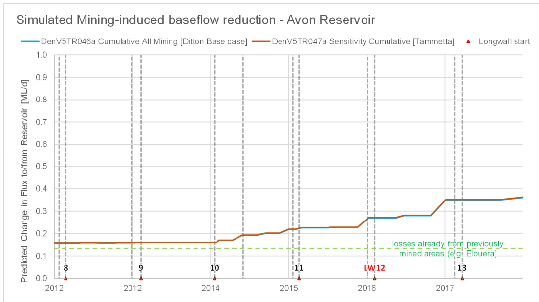
Figure 10. Model estimates of mine-induced reduction of baseflow to Lake Avon
