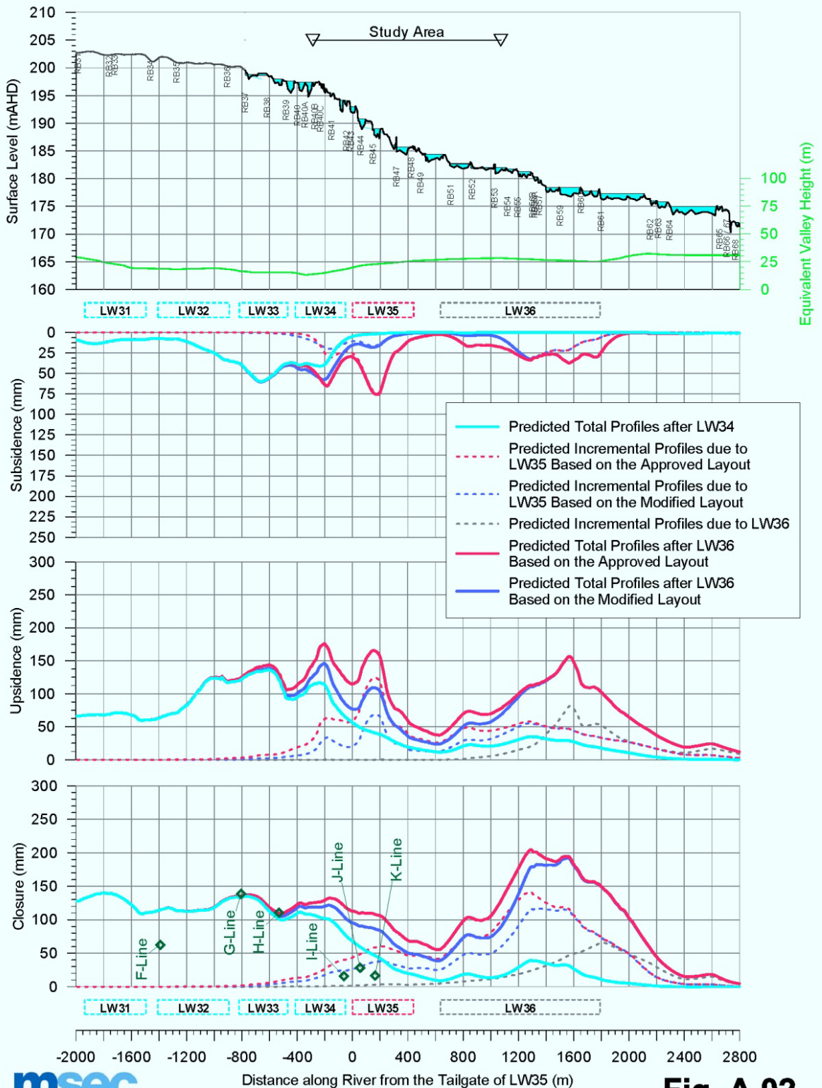
Figure 2. Predicted Profiles of Subsidence, Upsidence and Closure along the Georges River Resulting from the Extraction of Longwalls 29 to 36 (MSEC598).
