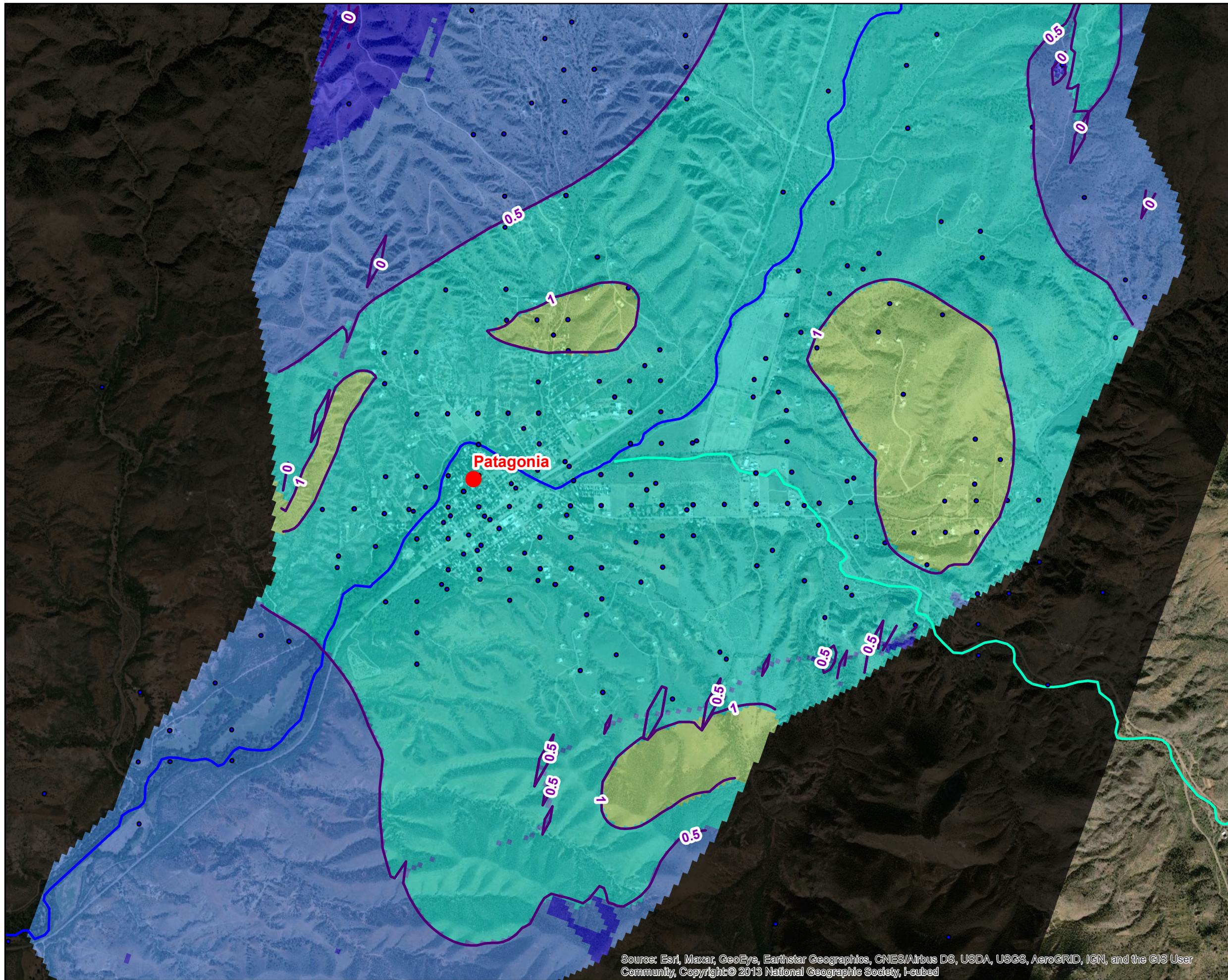
FIGURE 42 Residual Rise in Groundwater Levels after 10 Years (5 years of recovery) Patagonia Groundwater Model
